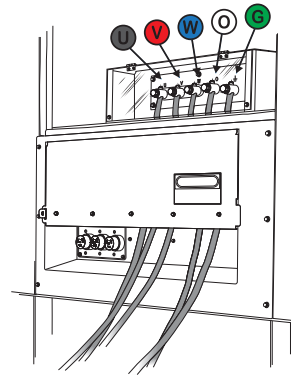
Generator Trailer
